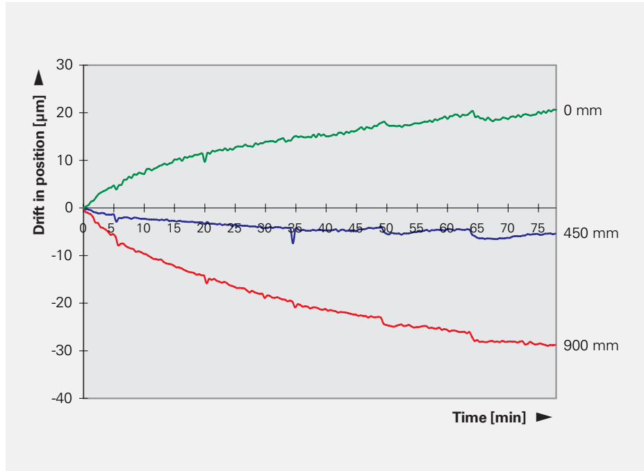
Fig. 10: Drift of three positions during positioning accuracy measurement in accordance with ISO/DIS 230-3 on a feed axis with a ball screw in fixed bearings at both ends. Position measurement via rotary encoder and ball screw causes a distinct drift of positions due to the thermal growth of the ball screw.
