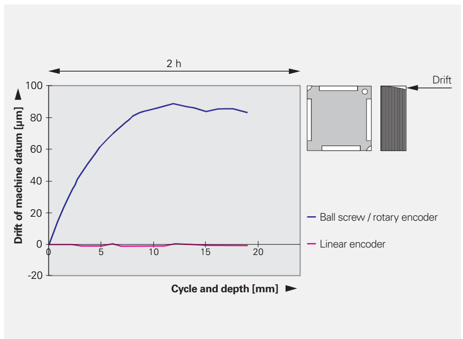
Fig. 9: Result of the experiment in Fig. 8. The left pocket of the workpiece plainly shows a step pattern resulting from thermal expansion of the ball screw.
