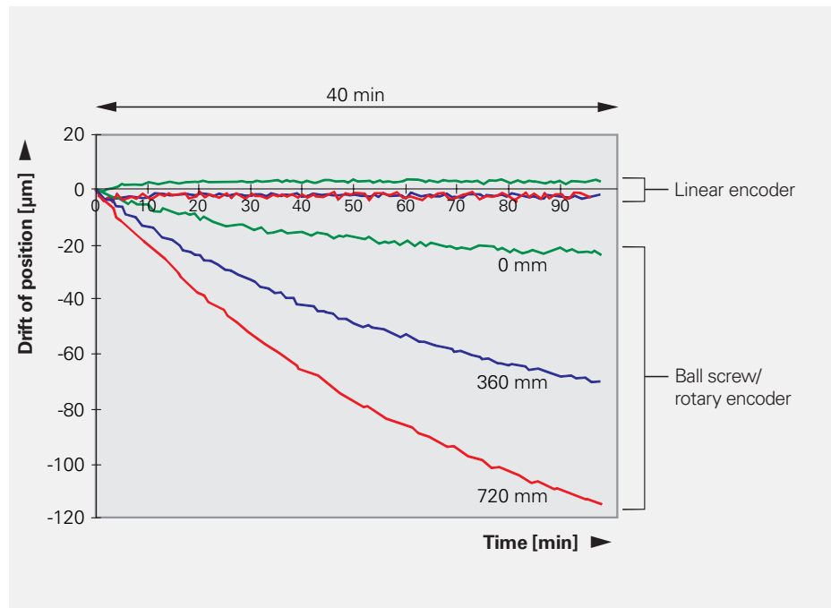
Fig. 7: Drift of three positions during positioning accuracy measurement in accordance with ISO/DIS 230-3 on a machining center with ball screw in fixed/floating bearings. Position measurement via rotary encoder and ball screw shows a distinct drift of positions due to the thermal growth of the screw.
