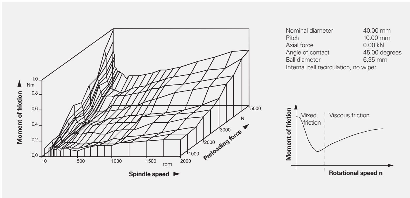
Fig. 4: Measured moment of friction of a two-point preloaded ball screw [4]. The Stribeck characteristics is plainly visible.
