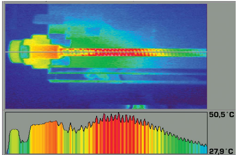
Fig. 12: Local heating of a ball screw in the traverse range of the ball nut after 6 hours of reciprocating traverse at 24 m/min between two positions separated by 150 mm [6]. For this thermographic snapshot, the machine table was moved aside at the end of the traverse program.
