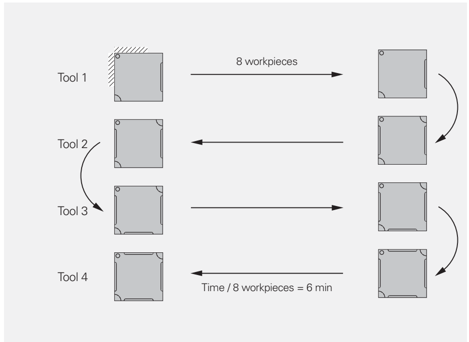
Fig. 8: Experimental setup for batch production with multiple workpieces. 4 pockets and 2 radii were machined using 4 tools with an infeed of 1 mm in the Z axis. To illustrate drift resulting from thermal expansion of the ball screw, the workpieces were not exchanged after machining. Instead, the part program was run repeatedly at successively increasing depth.
