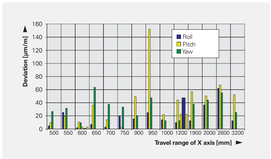
Fig. 16: Pitch, roll and yaw angles of feed axes of 16 different NC machines
